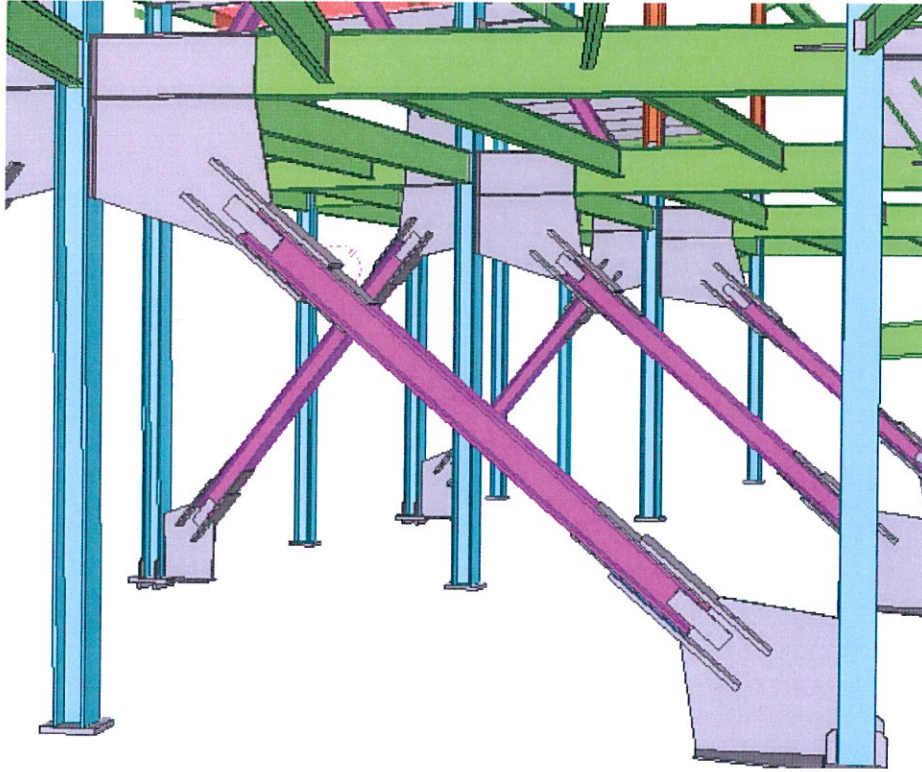
Figure 1: Perspective View of Braced Bay
